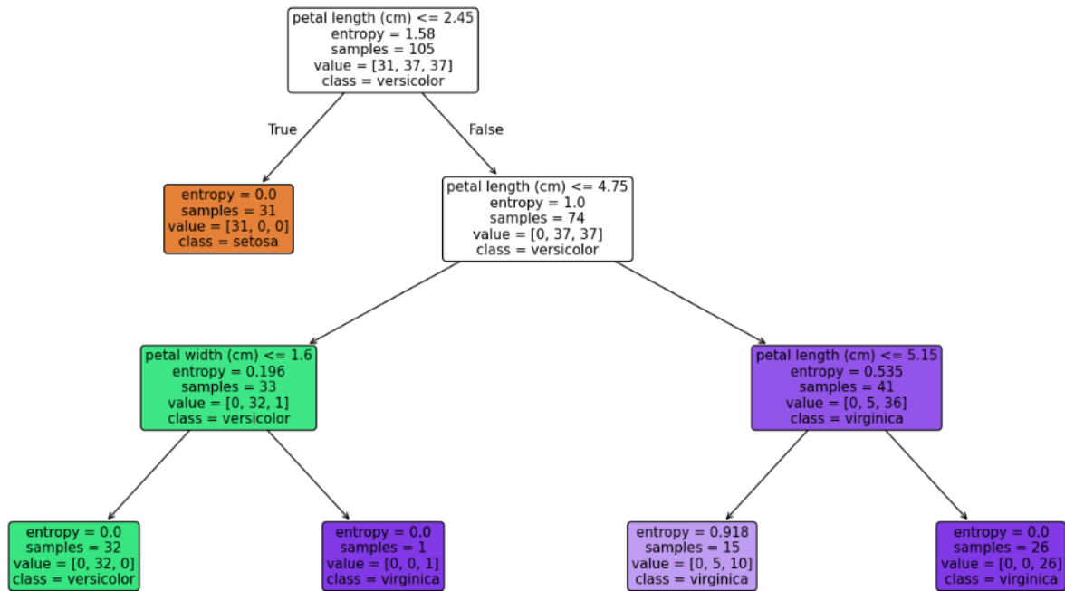
Decision Tree (Max Depth = 3)
